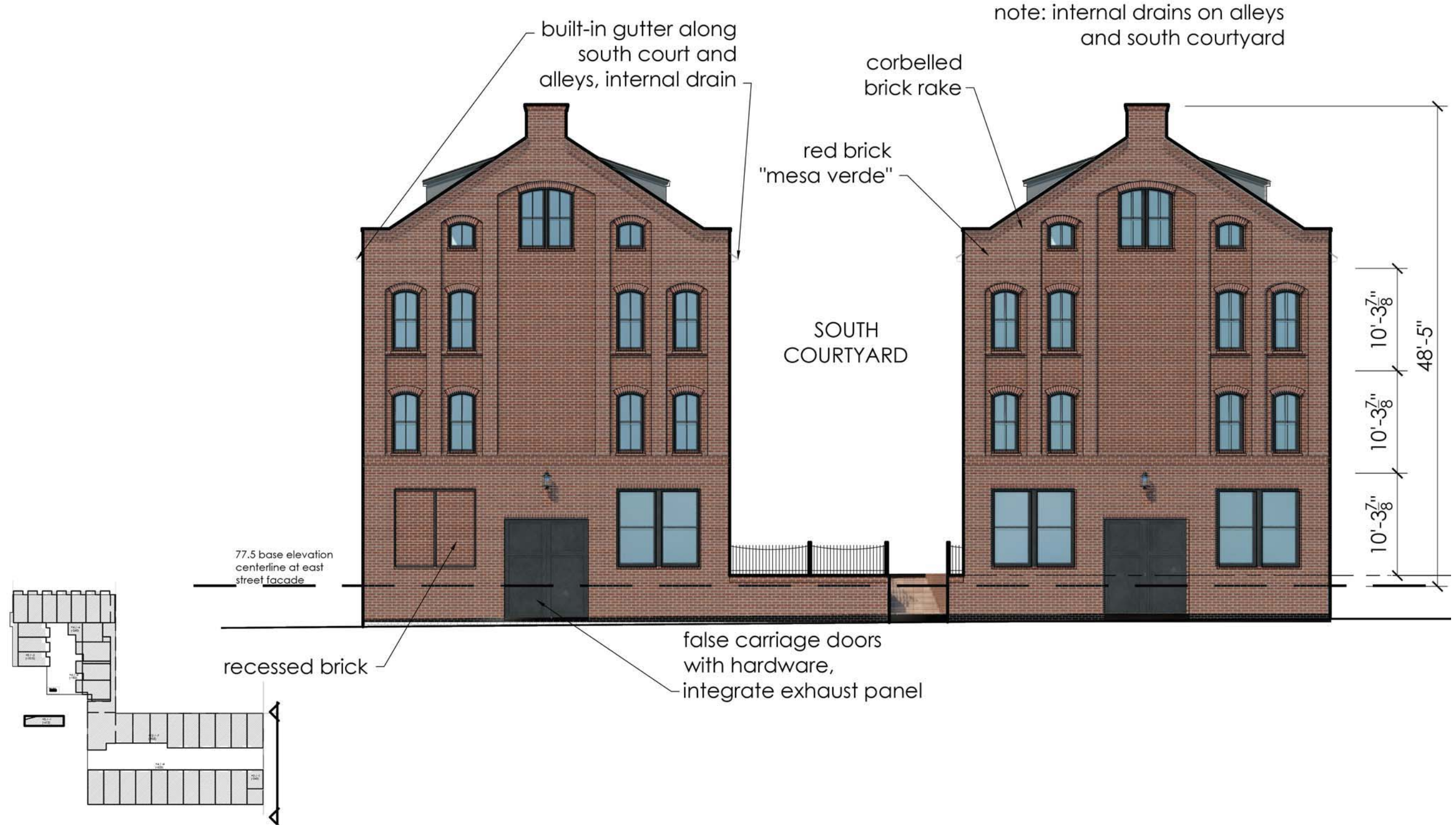
16' Alley elevation
